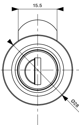
P9180 aluminium washer for glass panels
